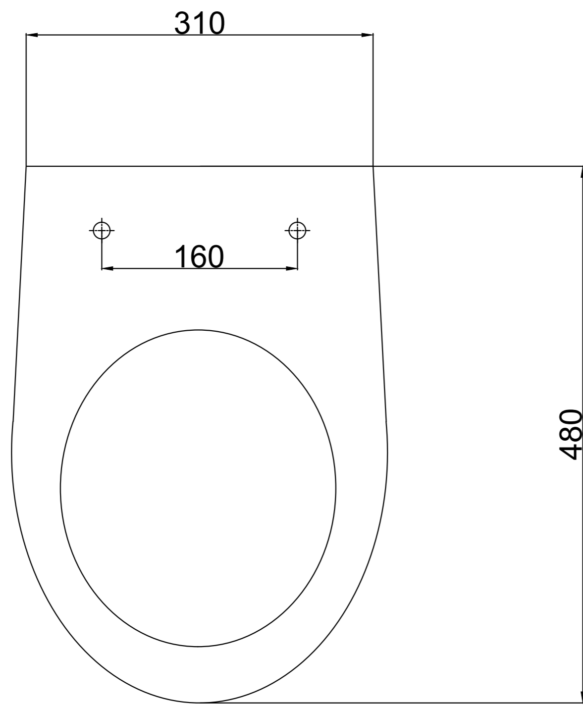
TOP VIEW
