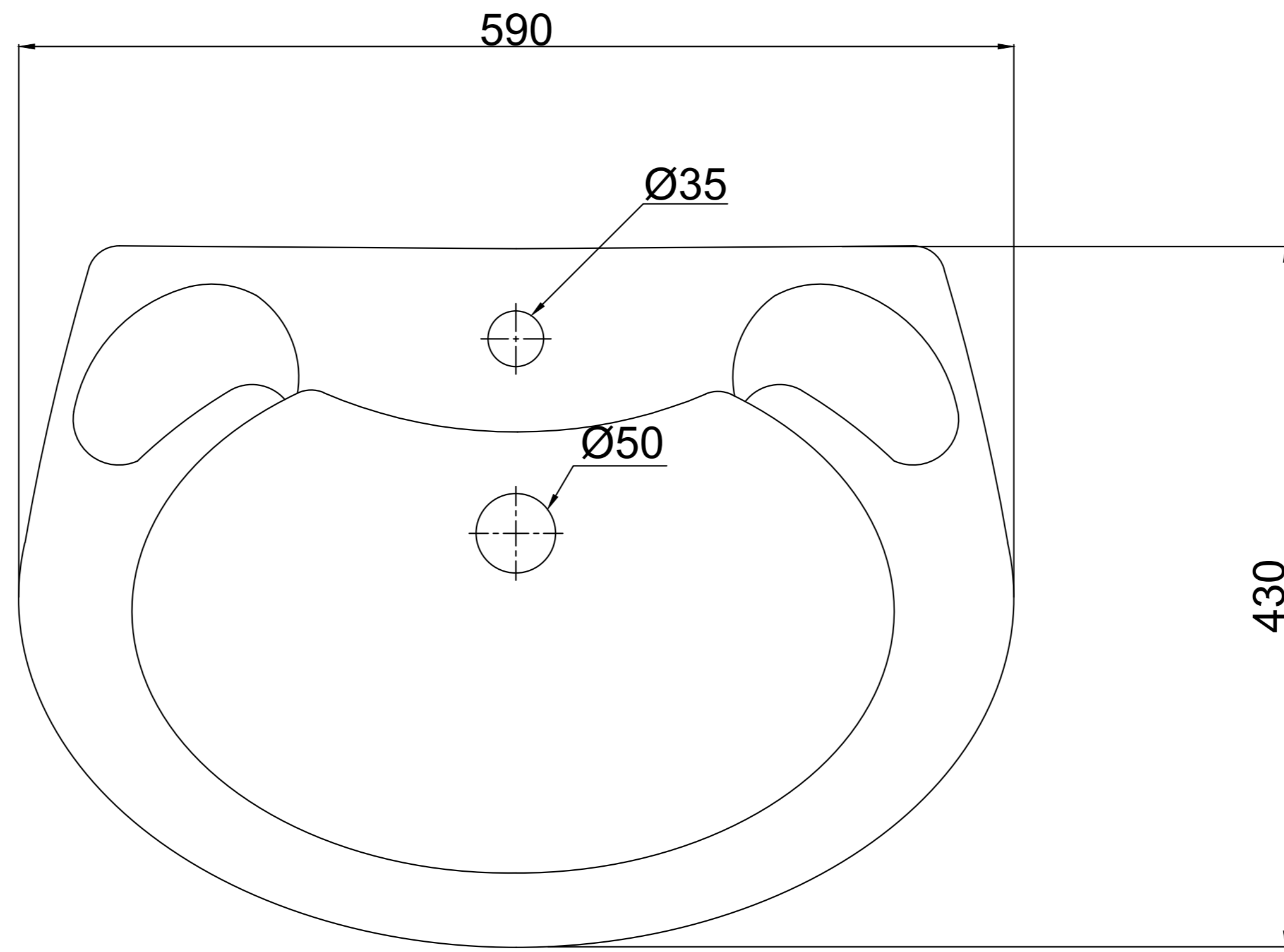
TOP VIEW
