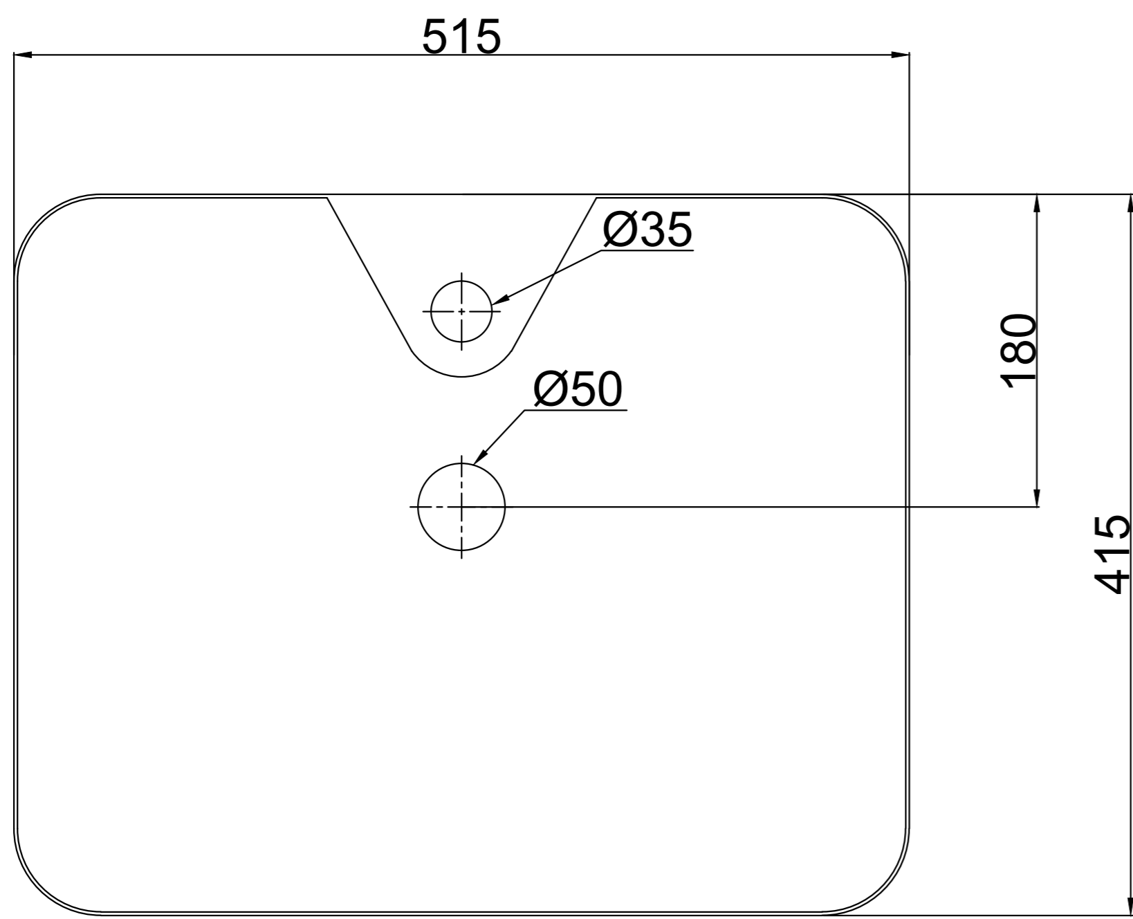
TOP VIEW
