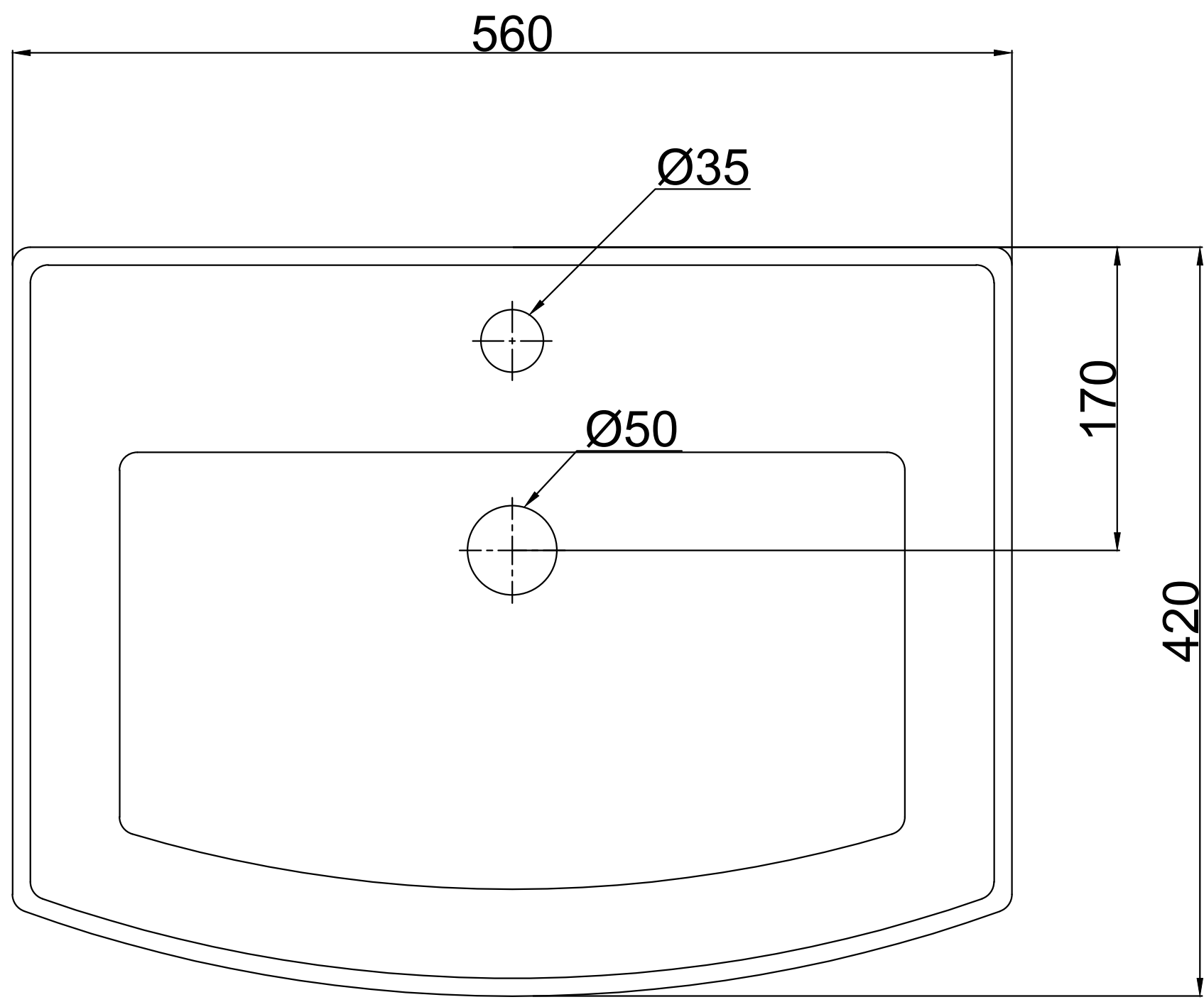
TOP VIEW
