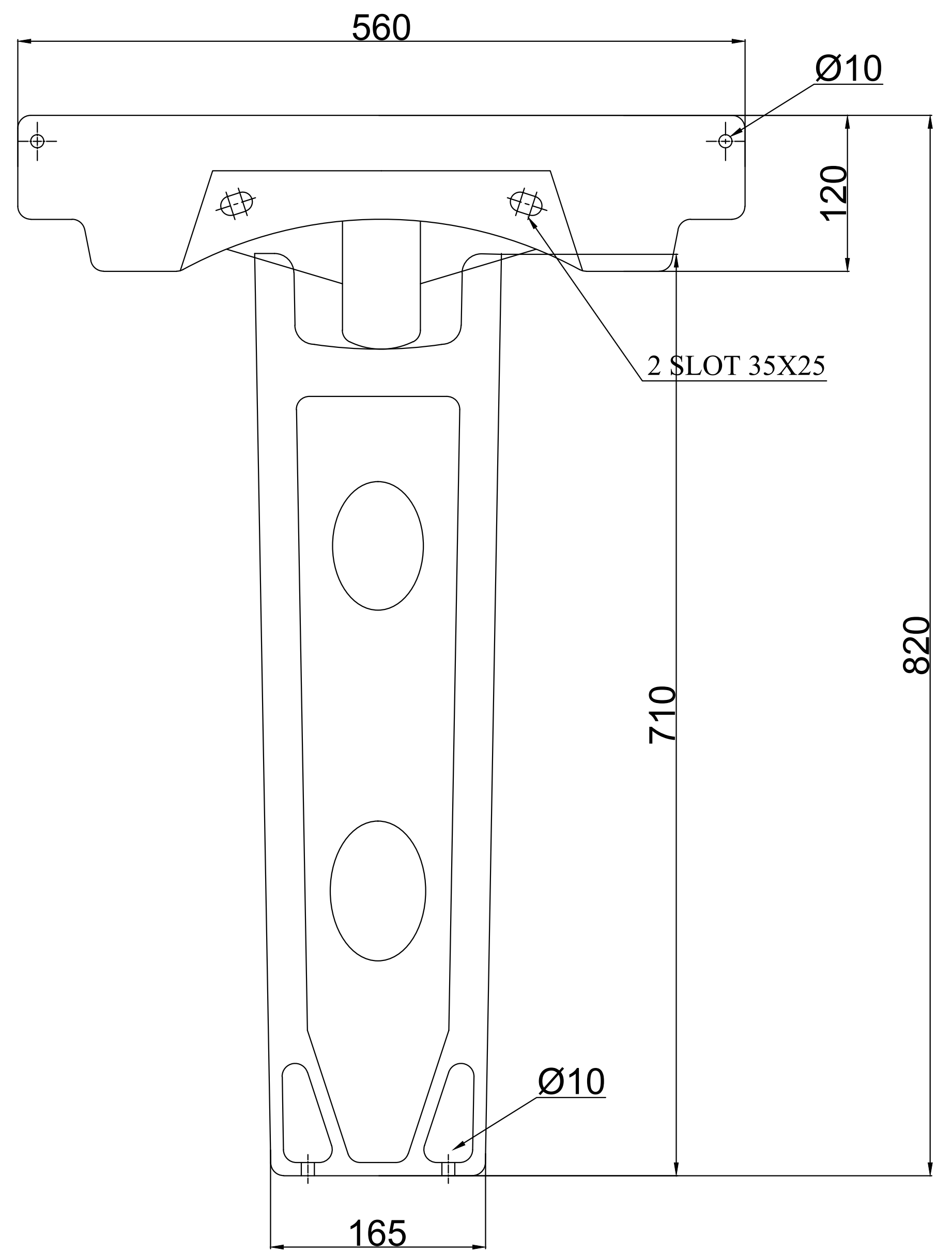
BACK VIEW
