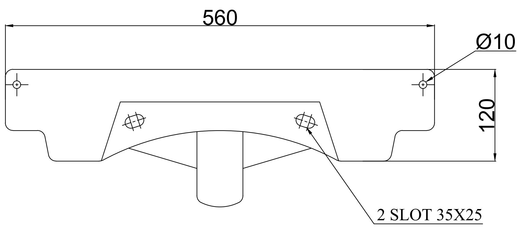
BACK VIEW
