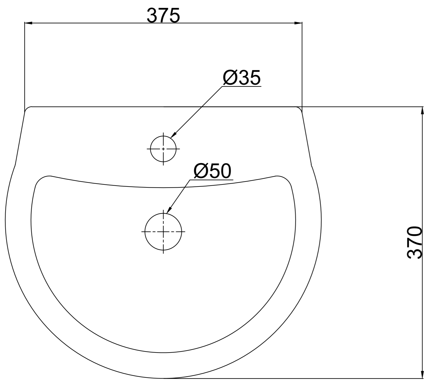
TOP VIEW
