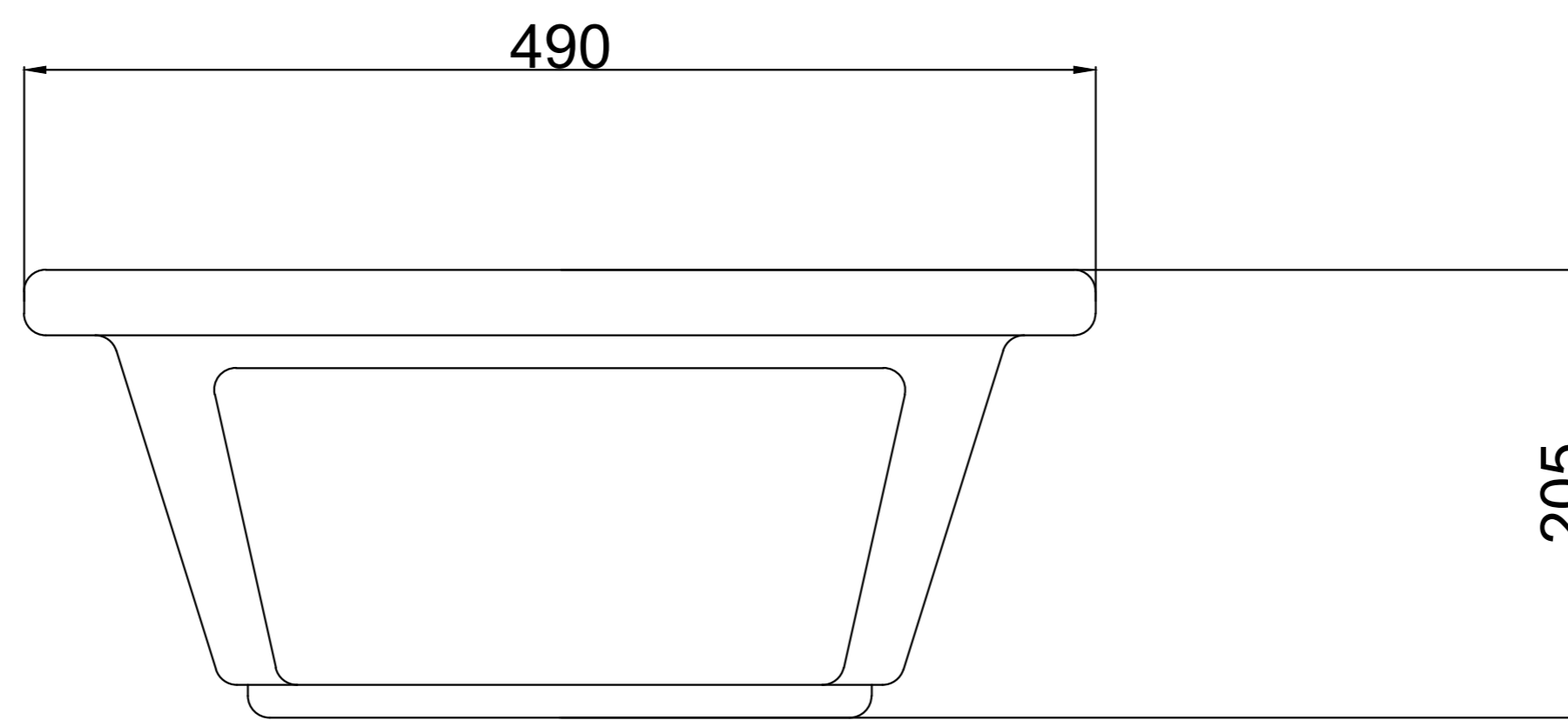
FRONT VIEW
