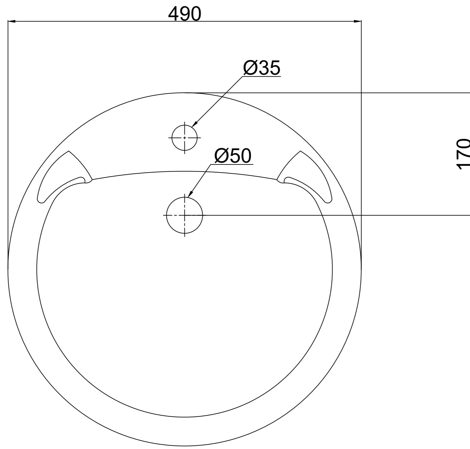
TOP VIEW
