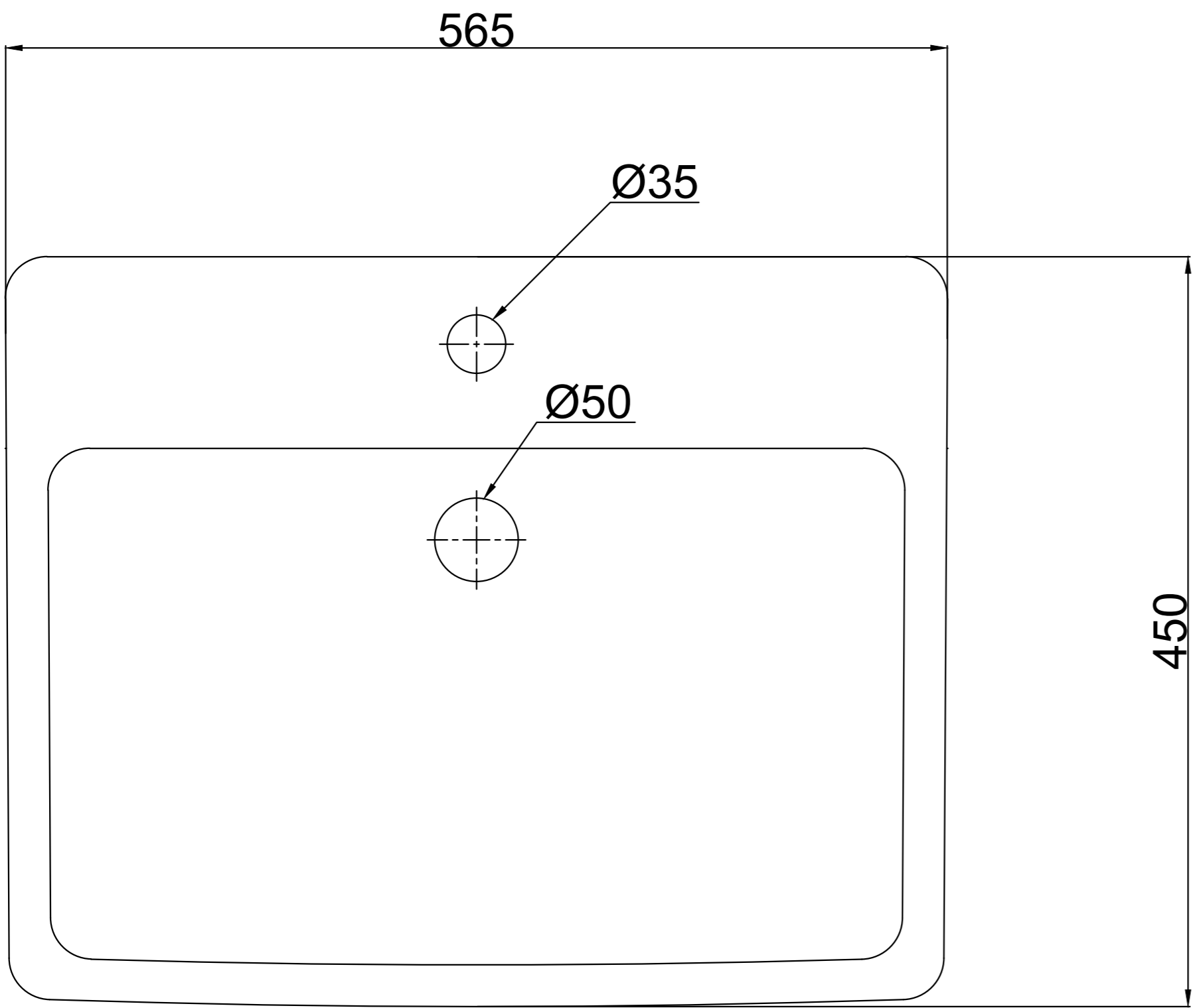
TOP VIEW
