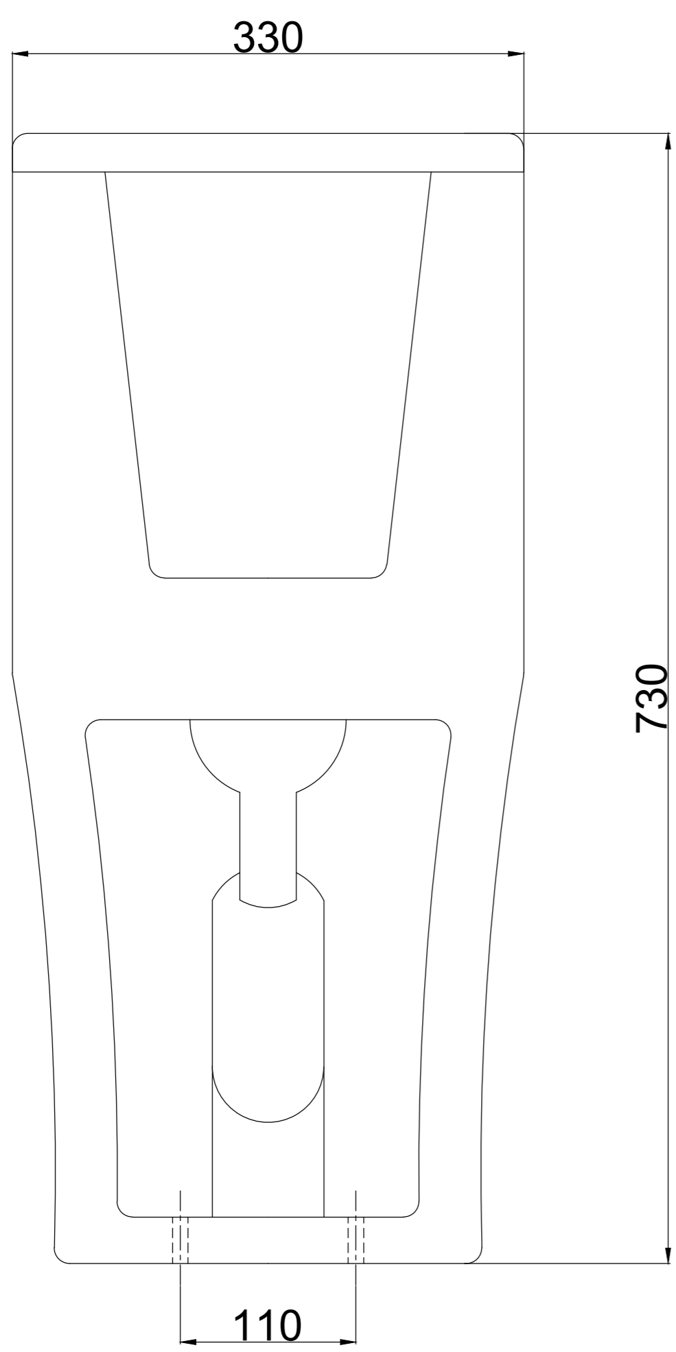
BACK VIEW
