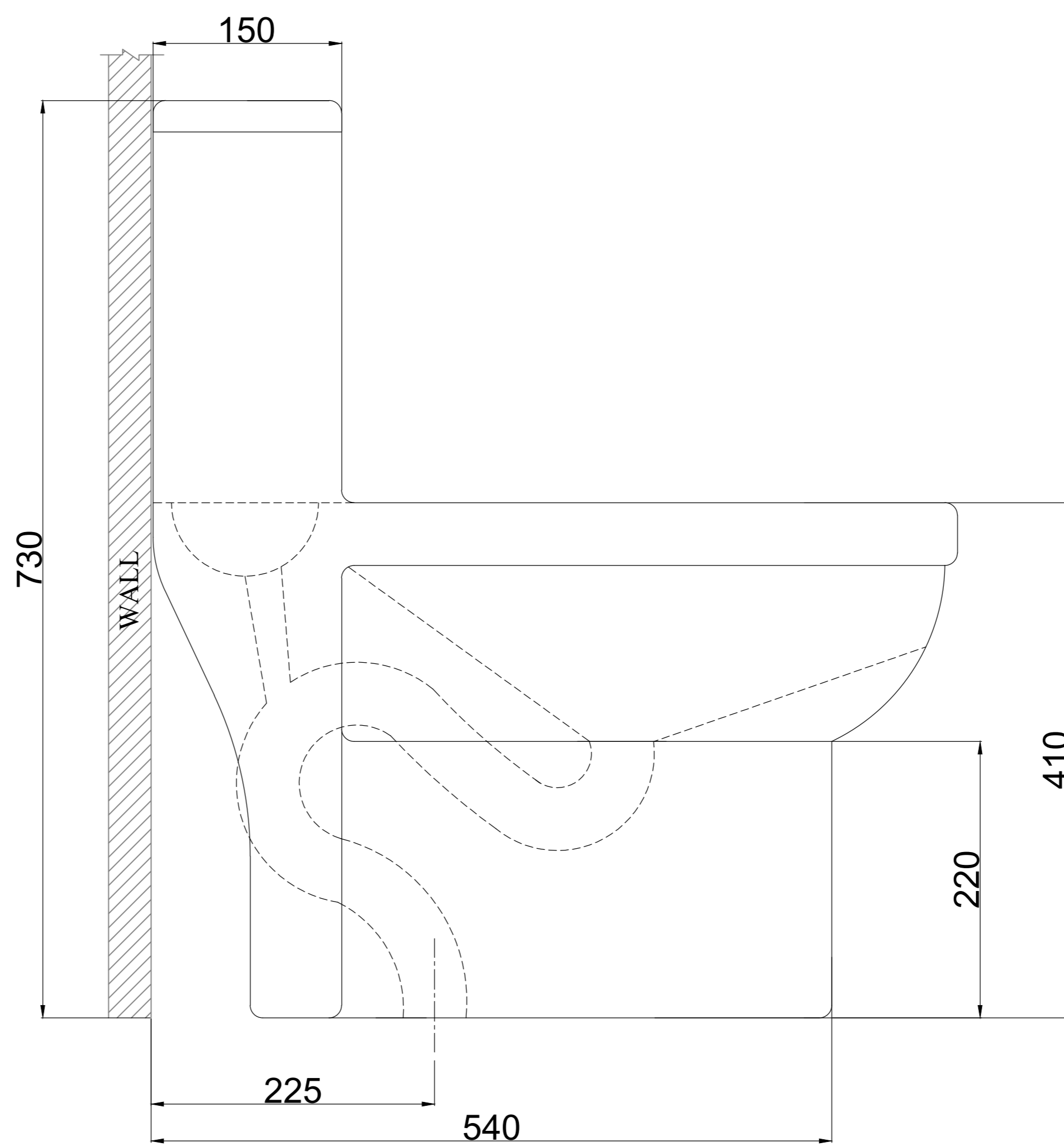
SIDE VIEW
