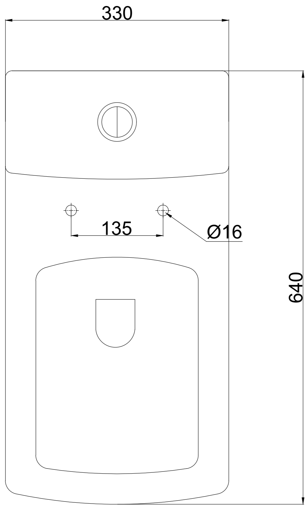
TOP VIEW
