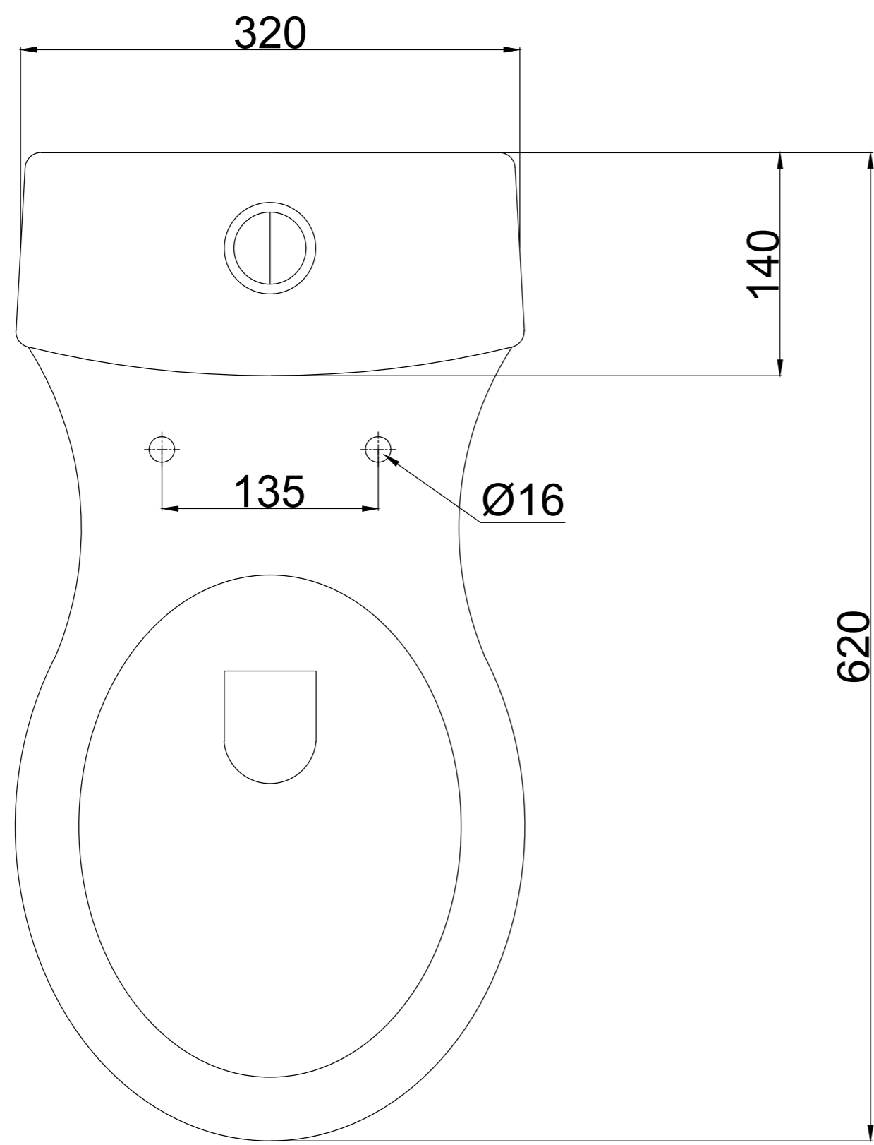
TOP VIEW
