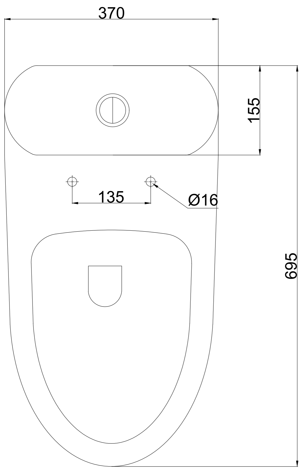
TOP VIEW
