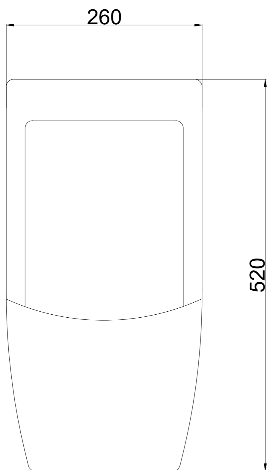
TOP VIEW
