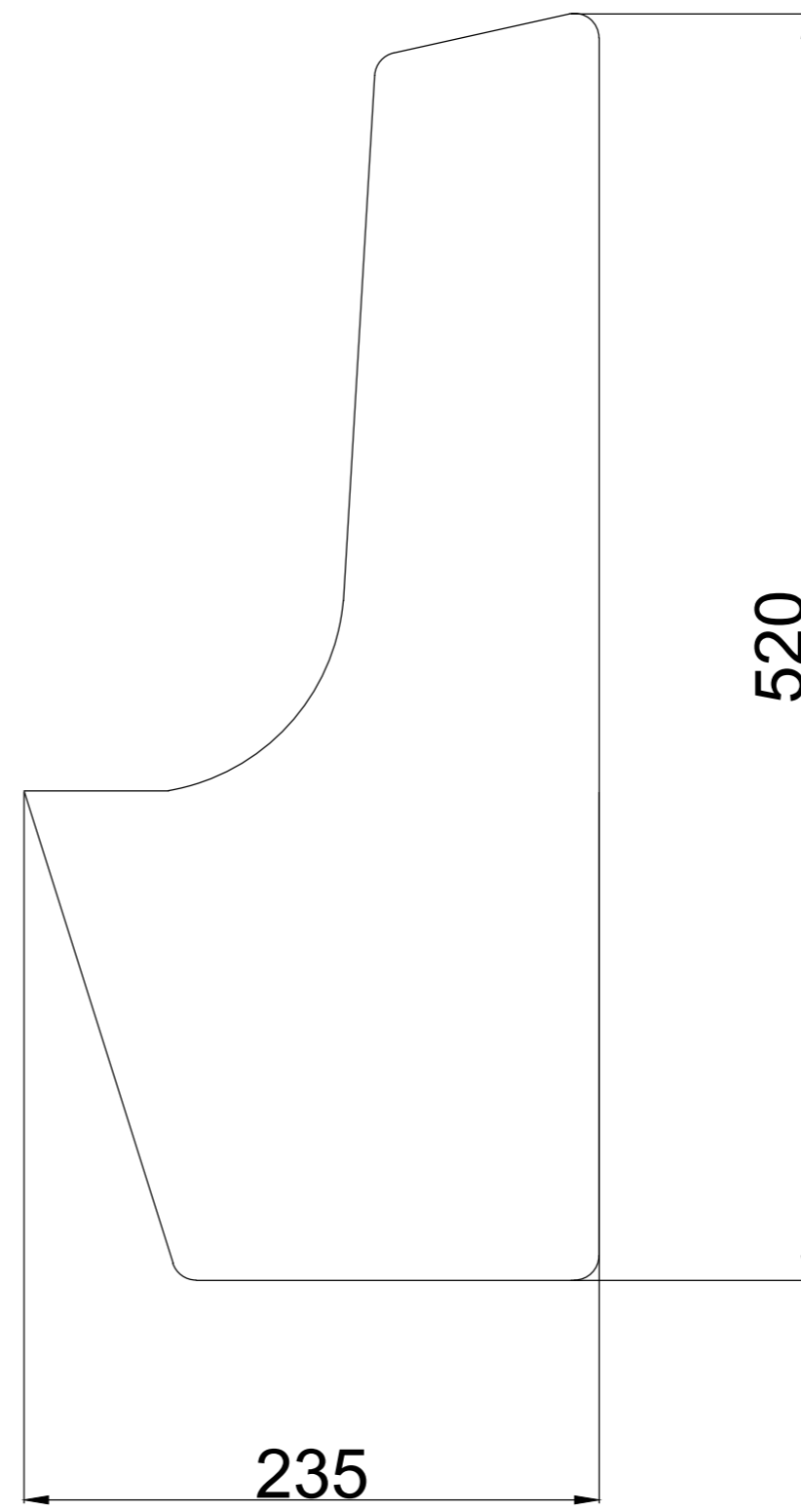
SIDE VIEW
