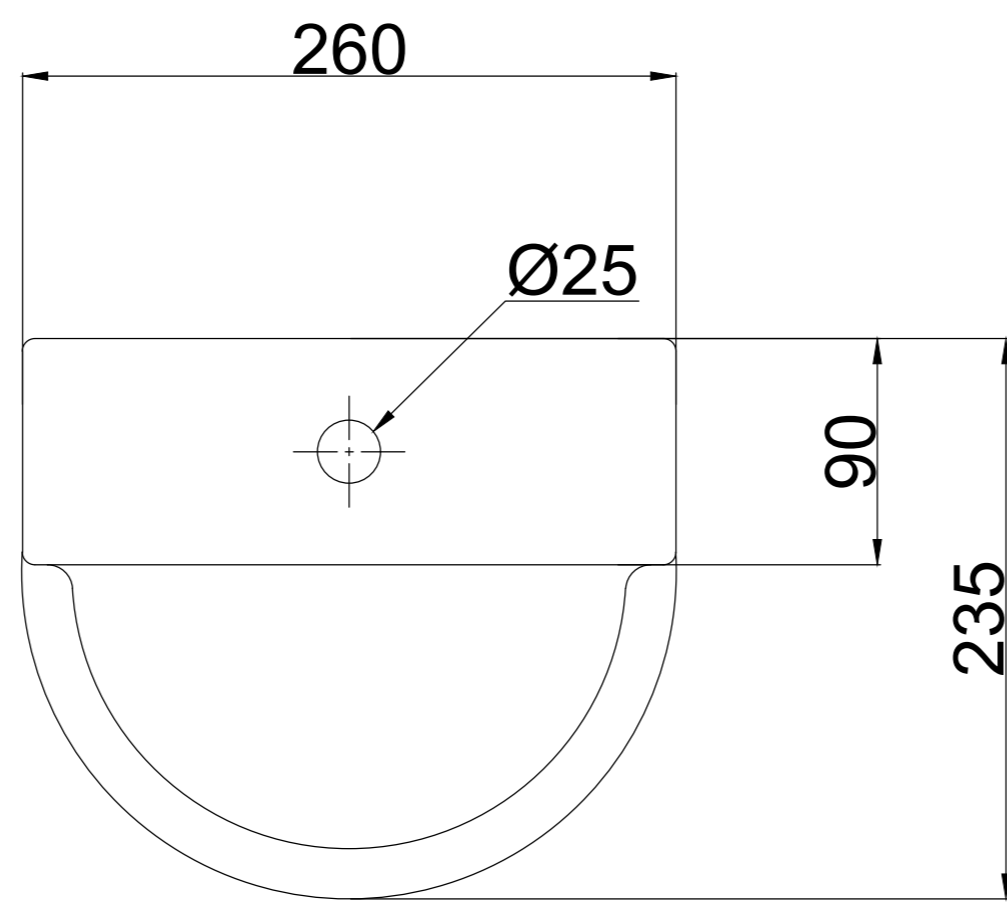
TOP VIEW
