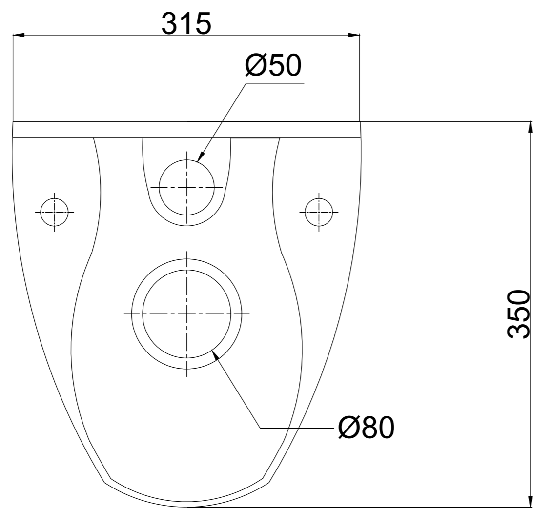
BACK VIEW
